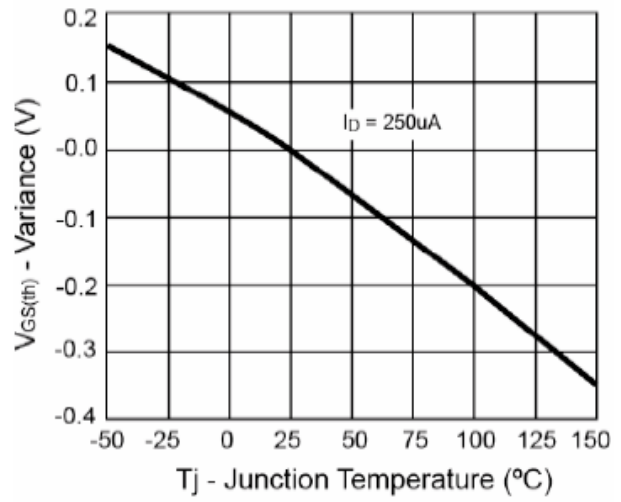
Fig.8 Threshold Voltage
