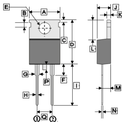
TO-220YA
