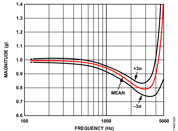
Figure 21. Magnitude/Frequency Response
