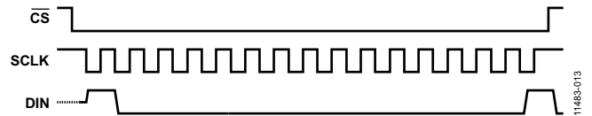
Figure 14. SPI Sequence for Selecting Page 1 for Access (DIN = 0x8001)
