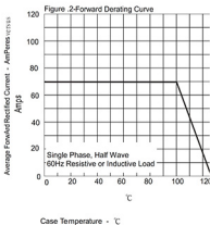
Figure 2-Forward Derating Curve
