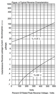
Figure 4-Typical Reverse Characteristics
