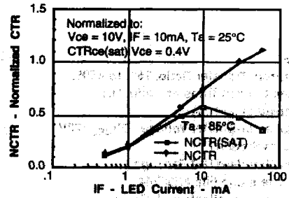
Figure 6. Collector-emitter current versus temperature and LED current
