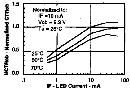
Figure 8. Normalized CTRcb versus LED current and temperature
