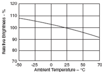
Fig. 1C. Relative Luminous Intensity vs. Temperature (See Note 2)
