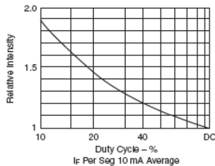
Fig. 1E. Relative Luminous Intensity vs. Duty Cycle
