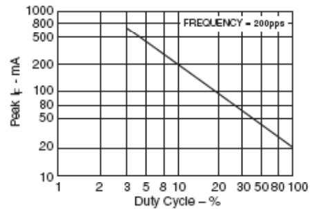
Fig. 3D. Max Peak Current vs. Duty Cycle
