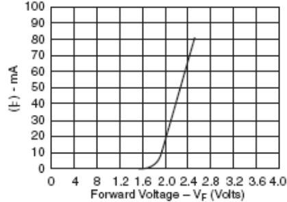
Fig. 4B. Forward Current vs. Forward Voltage
