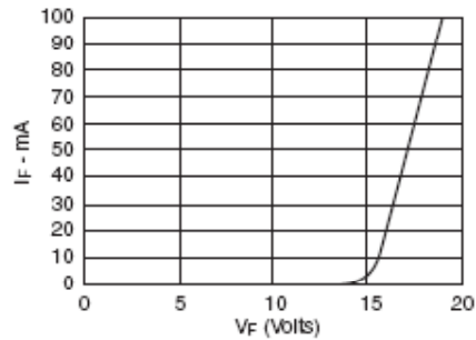
Fig. 3B. Forward Current vs. Forward Voltage
