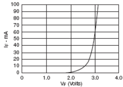
Fig. 1B. Forward Current vs. Forward Voltage
