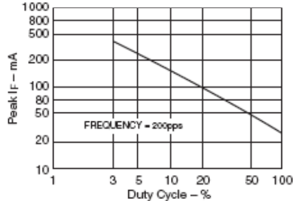
Fig. 4D. Maximum Peak Current vs. Duty Cycle
