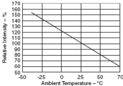
Fig. 3C. Relative Luminous Intensity vs. Temperature (See Note 2)
