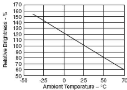
Fig. 3C. Relative Luminous Intensity vs. Temperature (See Note 2)
