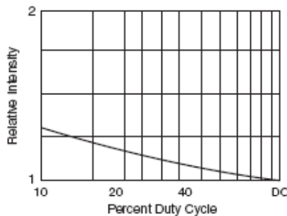
Fig. 3E. Relative Luminous Intensity vs. Duty Cycle
