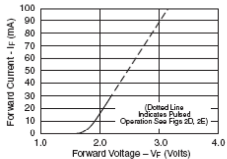
Fig. 2B. Forward Current vs. Forward Voltage
