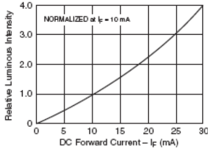
Fig. 4A. Relative Luminous Intensity vs. Forward Current
