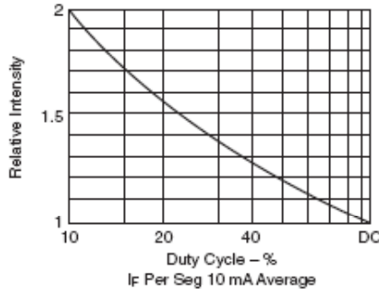
Fig. 4E. Relative Luminous Intensity vs. Duty Cycle
