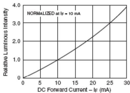
Fig. 2A. Relative Luminous Intensity vs. DC Forward Current
