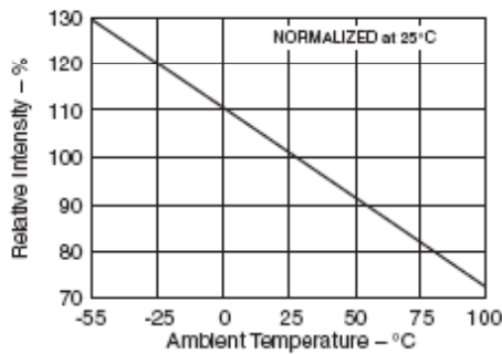
Fig. 2C. Relative Luminous Intensity vs. Temperature (See Note 2)
