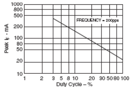
Fig. 1D. Max Peak Current vs. Duty Cycle
