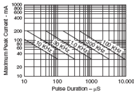
Fig. 2E. Maximum Peak Current vs. Pulse Duration
