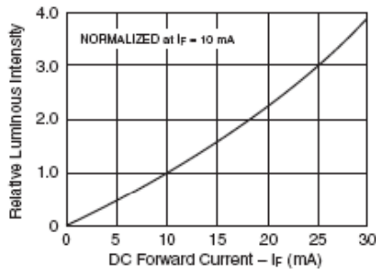
Fig. 1A. Relative Luminous Intensity vs. DC Forward Current
