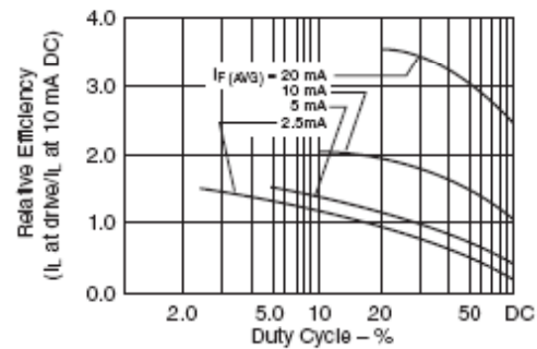
Fig. 2D. Relative Efficiency vs. Duty Cycle
