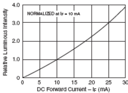
Fig. 3A. Relative Luminous Intensity vs. DC Forward Current
