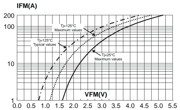
Fig. 2: Forward voltage drop versus current (per diode).
