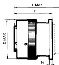
Plug Assembly
