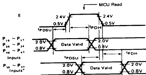
Figure 3 Data Set-up and Hold Times (MCU Read)
