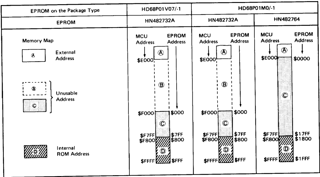
Figure 27 Memory Map When Emulating the HD6801S0
