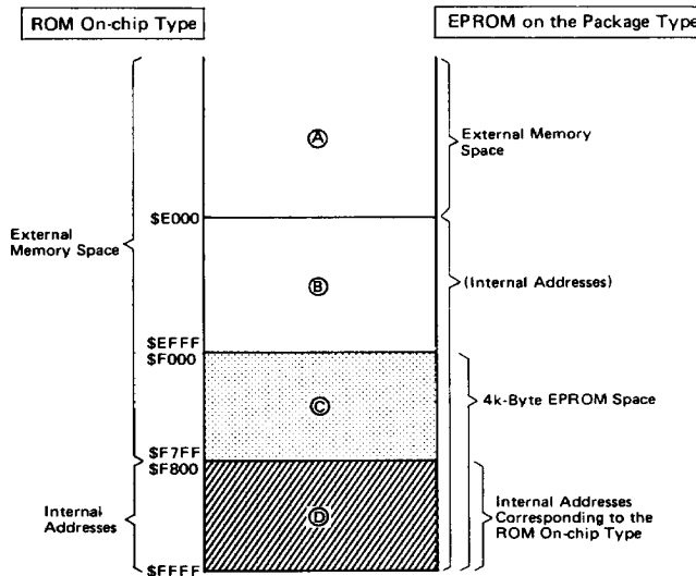
Figure 26 Memory Map Example when Emulating the HD6801S0 with the HD68P01M0 and the 4k-Byte EPROM
