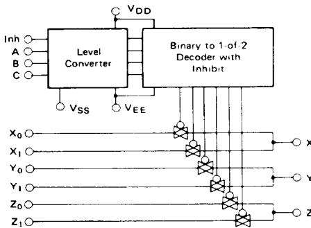
Figure 22 HD14053B Multiplexers/Demultiplexers
