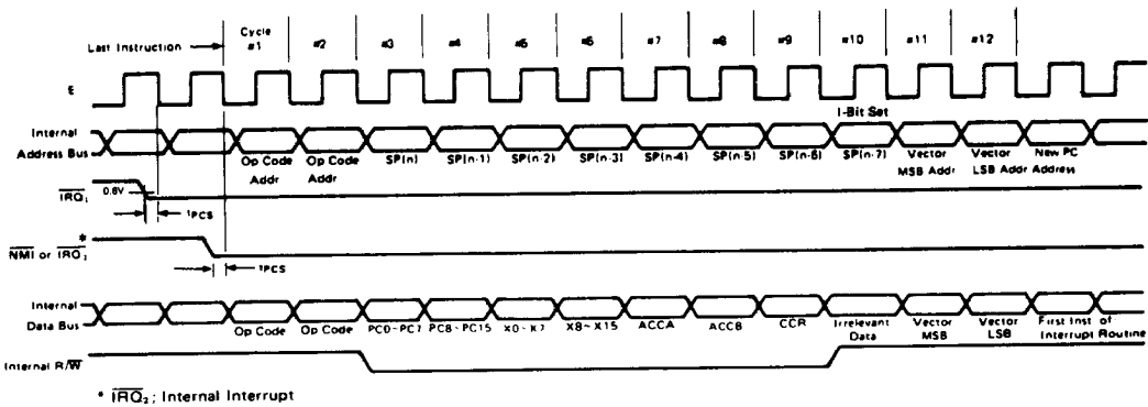
Figure 11 Interrupt Sequence
