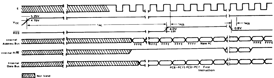
Figure 12 Reset Timing
