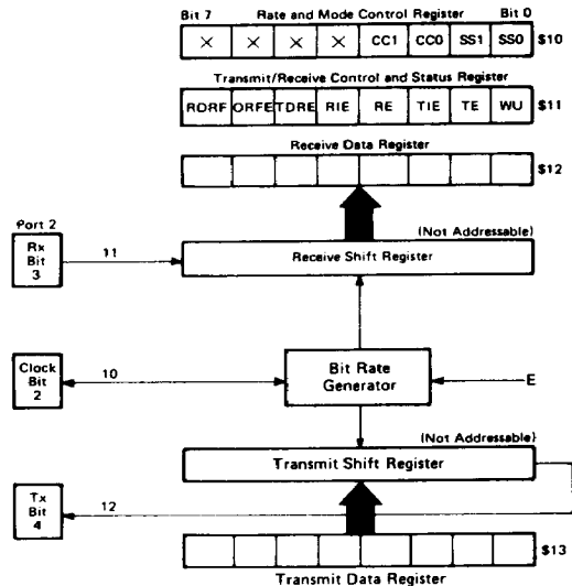
Figure 25 SCI Registers
