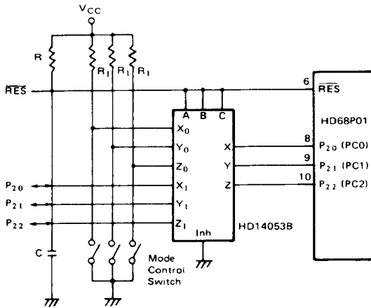
Figure 21 Recommended Circuit for Mode Selection
