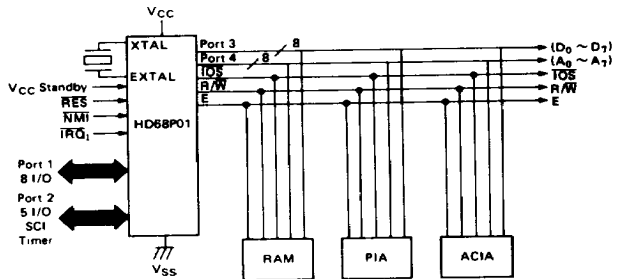
Figure 18 Expanded Non-Multiplexed Configuration
