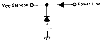
Figure 14 Battery Backup for V CC Standby
