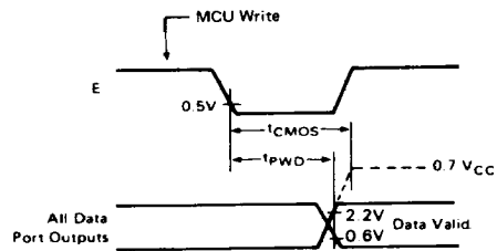
Figure 2 Expanded Non-Multiplexed Bus Timing
