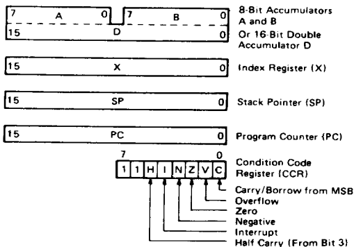
Figure 10 HD68P01 Programming Model
