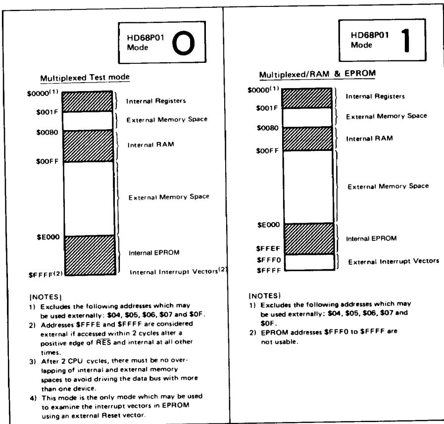
Figure 23 HD68P01 Memory Maps
