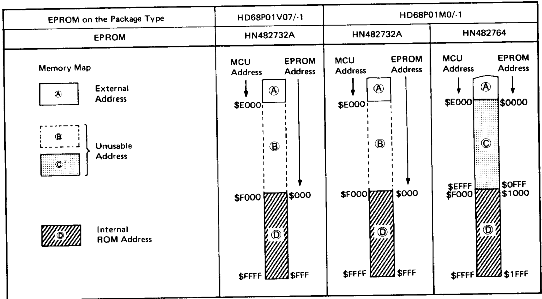
Figure 28 Memory Map When Emulating the HD6801V0
