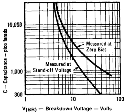
FIGURE 5 Typical Capacitance vs. Breakdown Voltage (Bidirectional Types)
