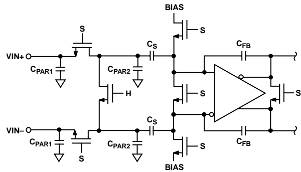
Figure 48. Switched-Capacitor Input
