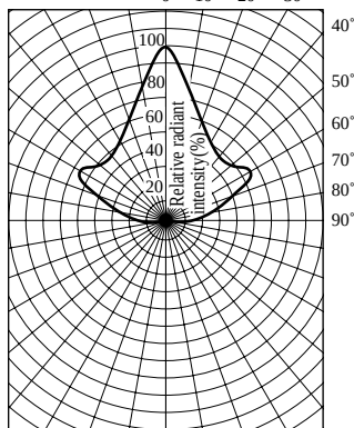
Directivity characteristics
