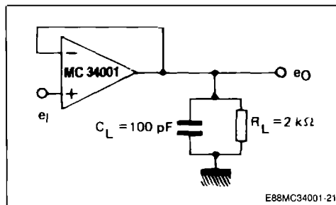
Figure 1 : Voltage Follower.
