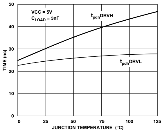
Figure 11. DRVH and DRVL t_{pdh} vs. Temperature
