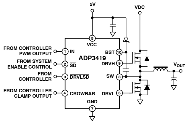
Figure 2. General Application Circuit
