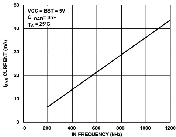
Figure 14. Supply Current vs. Frequency
