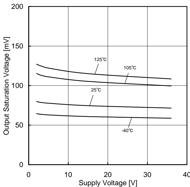
Figure 68. Output Saturation Voltage vs Supply Voltage (I OL =4mA)
