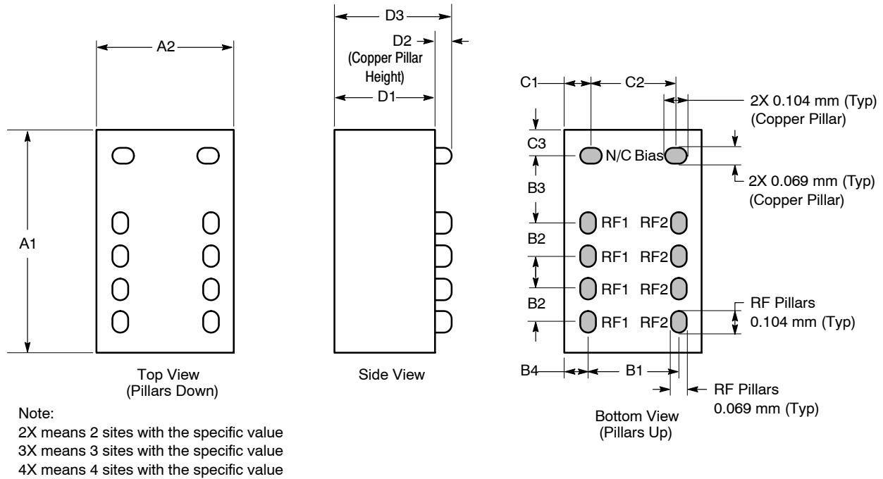
Figure 7. WLCSP Pin Markers and Dimensions
