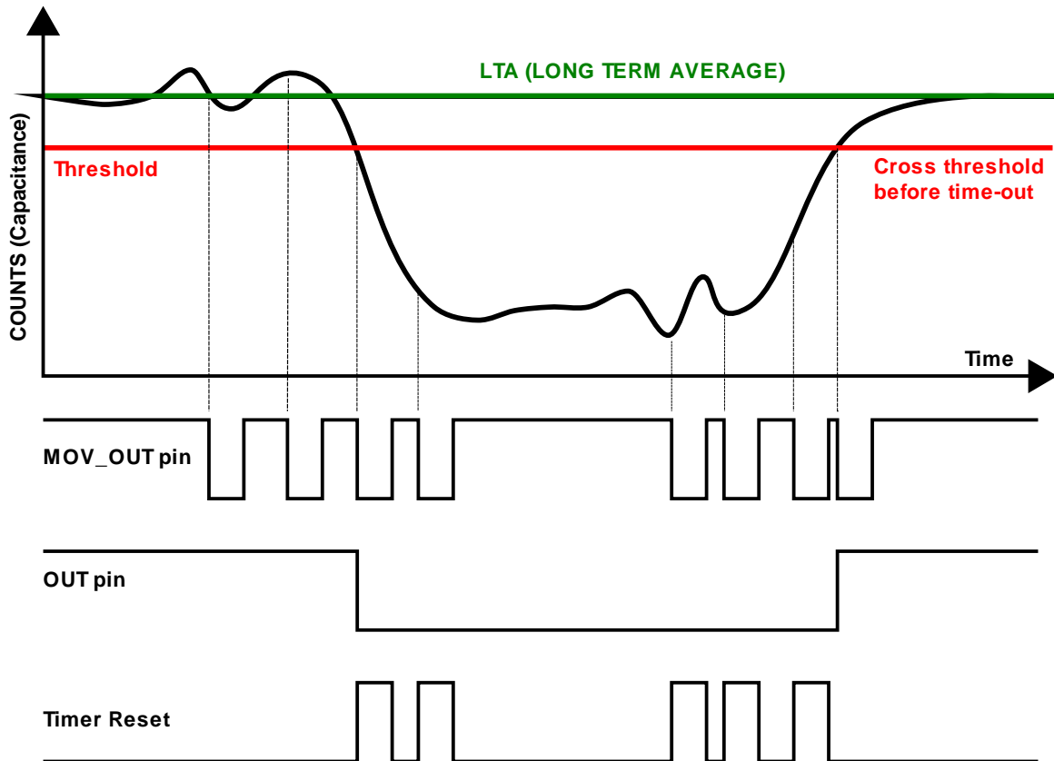
Figure 1.2 Plot of IQS229 streaming data along with the digital response
