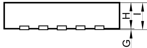
Figure 8.2 DFN-10 Package dimensions (side)
