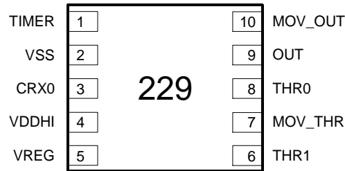
Figure 2.1 IQS229 pin-out (DFN10 package)
