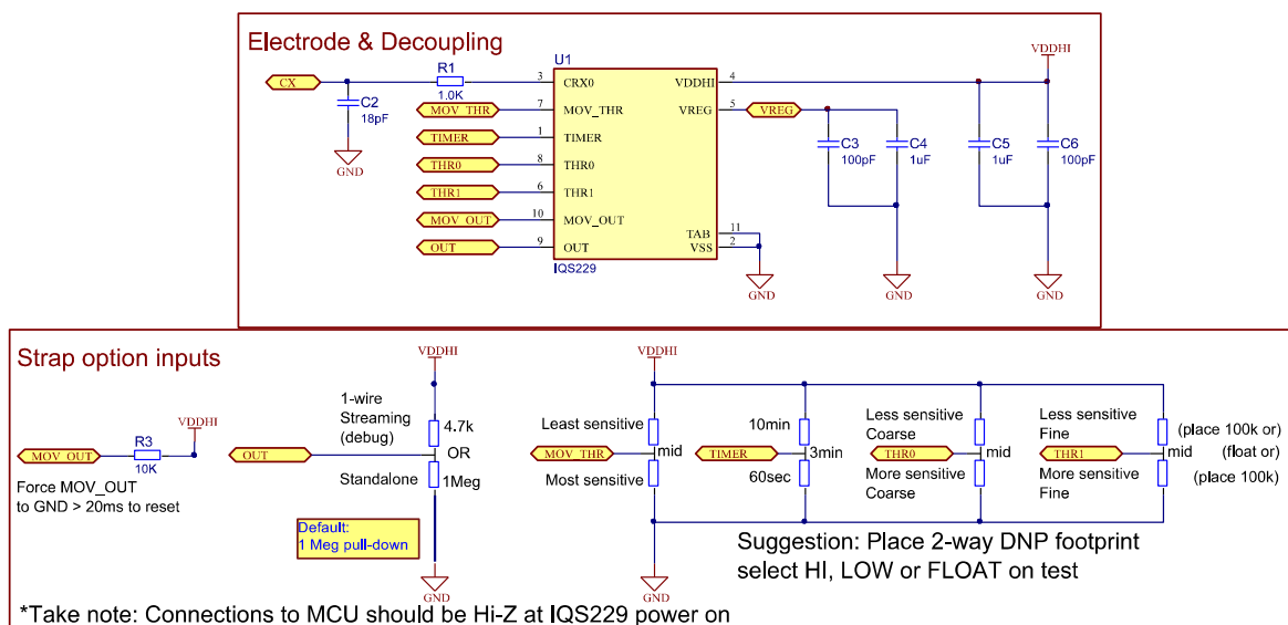
Figure 3.1 Reference schematic
