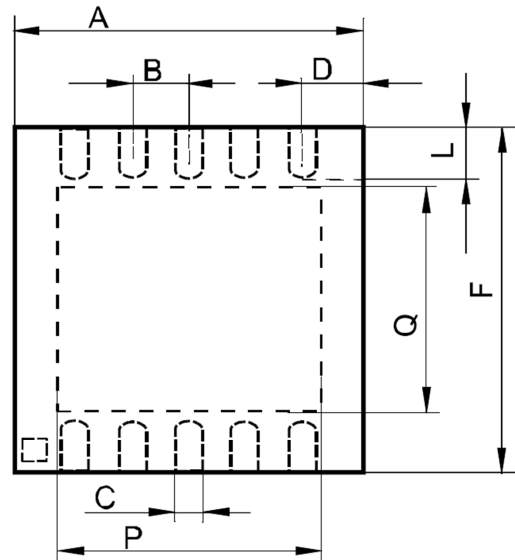
Figure 8.1 DFN-10 Package dimensions (bottom)
