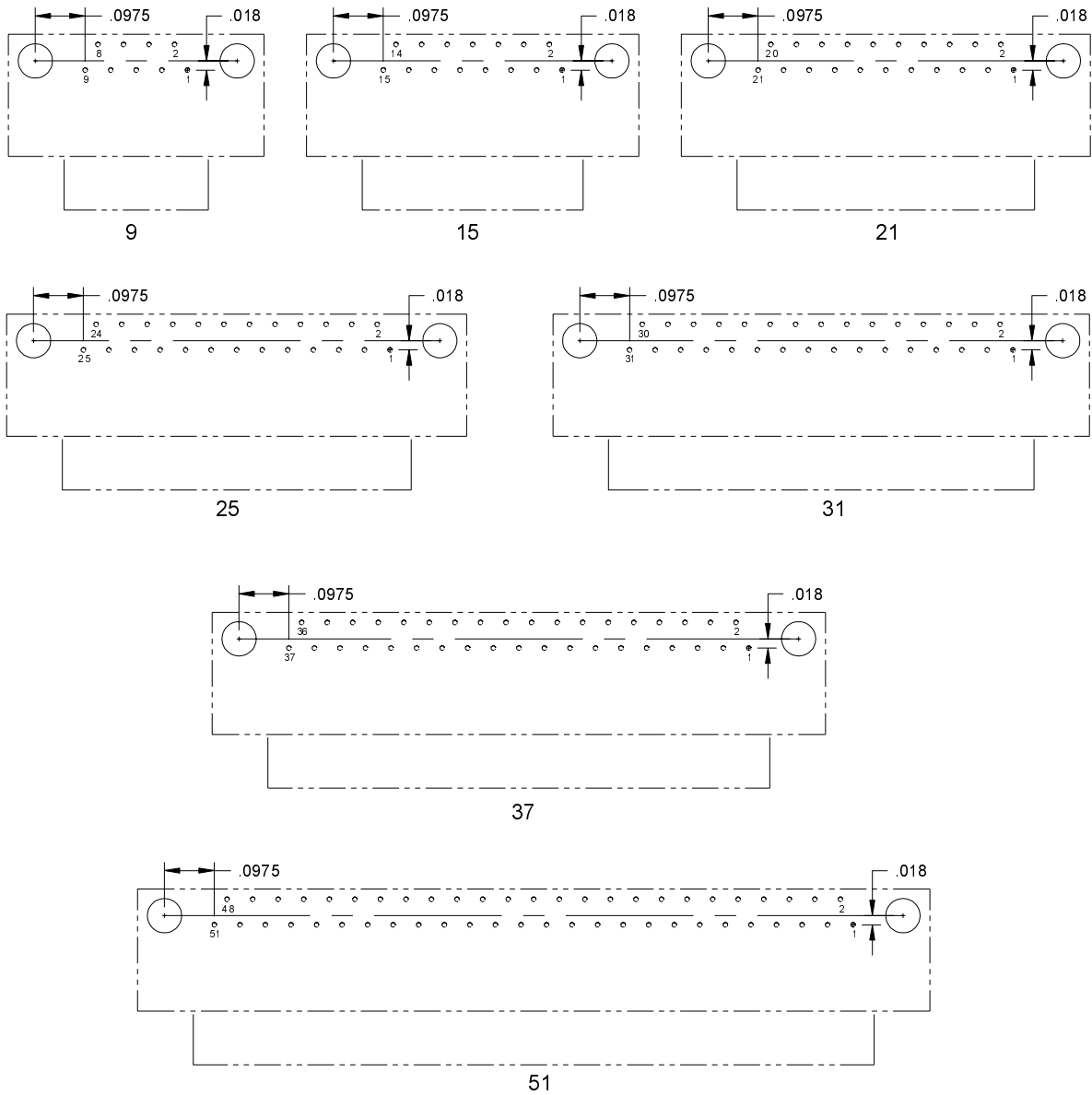
BRN1 PLUG PCB LAYOUTS (BOTTOM VIEW OF RECEPTACLE) .050 X .050 GRID PATTERN OFFSET .025
