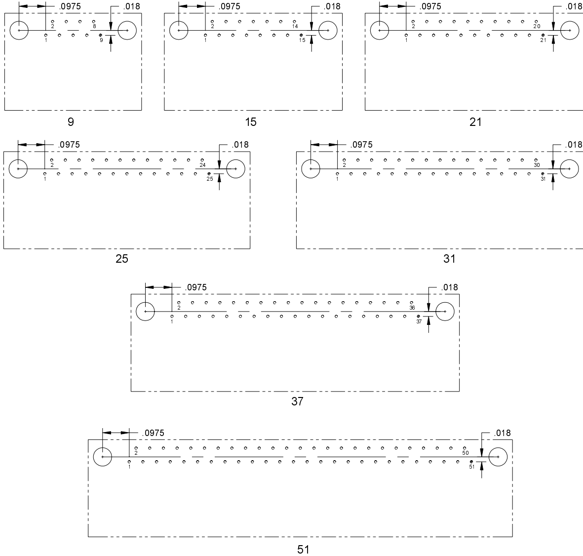
BRN1 RECEPTACLE PCB LAYOUTS (BOTTOM VIEW OF PLUG) .050 X .050 GRID PATTERN OFFSET .025
