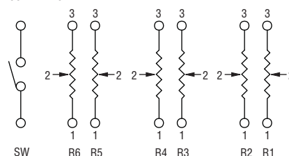
SCHEMATIC
