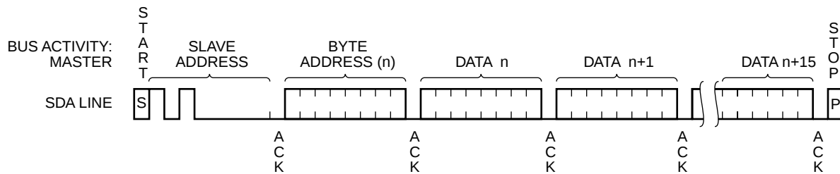
Figure 9. Page Write Timing
