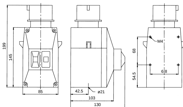
Moulded Enclosure for 5-pole CEE-plug MU25A-GC1
