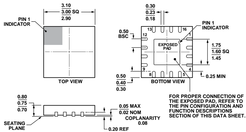
Figure 41. 16-Lead Lead Frame Chip Scale Package [LFCSF_WQ] 3 mm × 3 mm Body, Very Very Thin Quad (CP-16-22) Dimensions shown in millimeters
