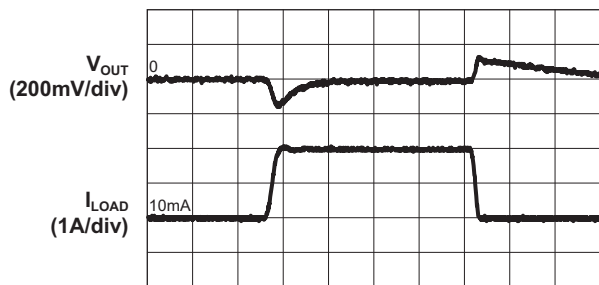
Step-Down Converter Load Transient
