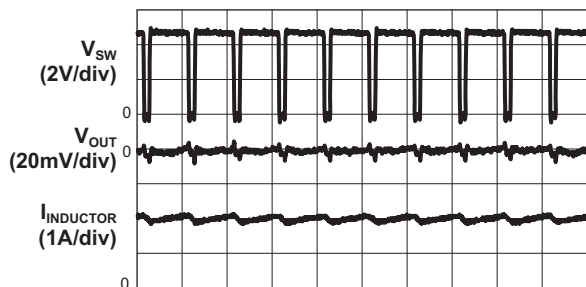
Step-Down Converter Output Ripple
