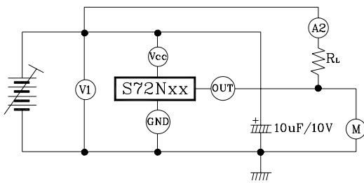
Test Circuit 1
