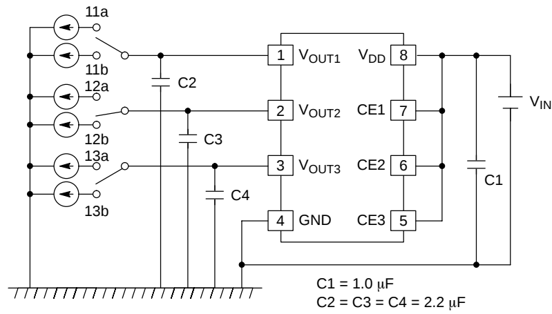
Figure 6. Test Circuit for Load Transient Response
