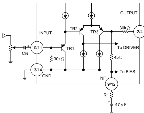
FOR HSIP-15A PACKAGE
