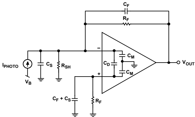
Figure 47. Wideband Photomultiplier Preamplifier
