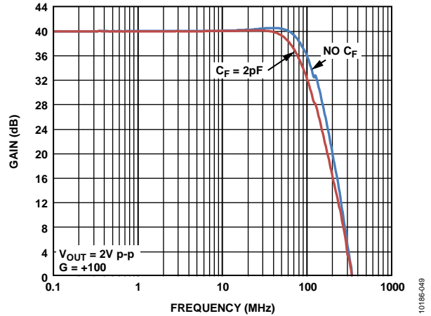
Figure 46. Large Signal Frequency Response, G = +100 , V_S = \pm 5\text{ V}
