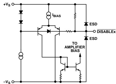
Figure 38. DISABLEx Circuit
