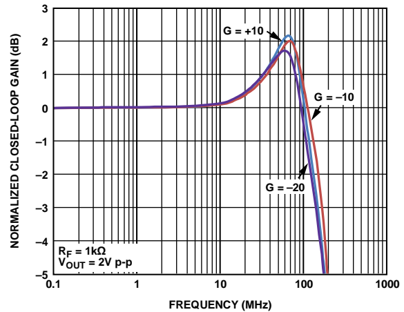
Figure 9. Large Signal Frequency Response vs. Gain
