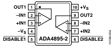
Figure 4. Pin Configuration
