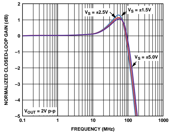
Figure 8. Large Signal Frequency Response vs. Supply Voltage
