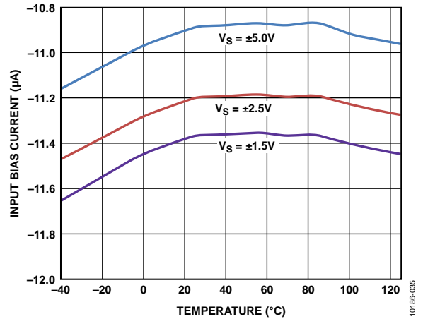
Figure 32. Input Bias Current vs. Temperature for Various Supplies
