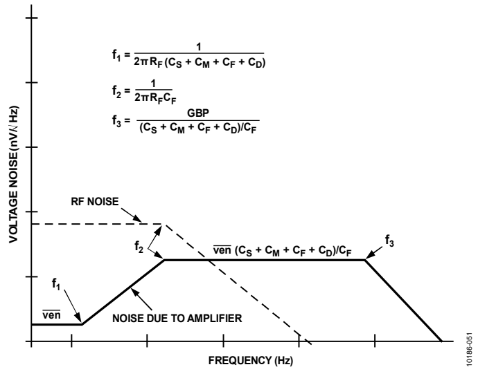
Figure 48. Photomultiplier Voltage Noise Contributions
