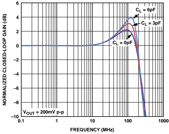
Figure 11. Small Signal Frequency Response vs. Capacitive Load
