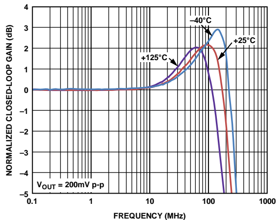
Figure 7. Small Signal Frequency Response vs. Temperature
