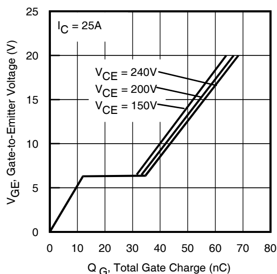
Fig 14. Typical Gate Charge vs. Gate-to-Emitter Voltage
