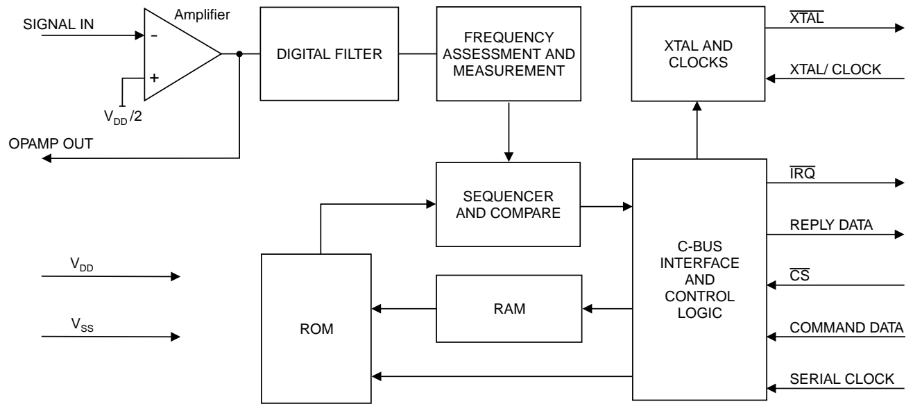
Figure 1: Block Diagram
