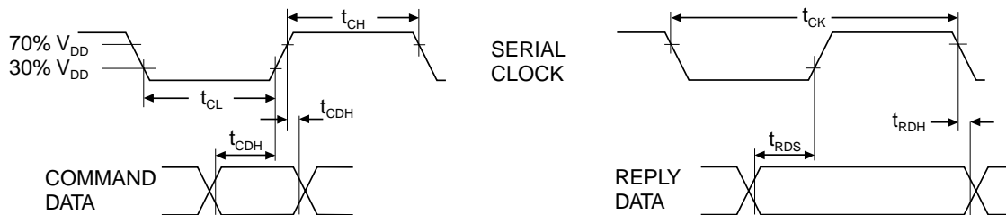
Figure 3: C-BUS Timing
