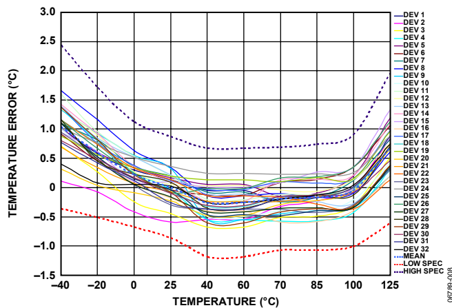
Figure 6. Local Temperature Sensor Error
