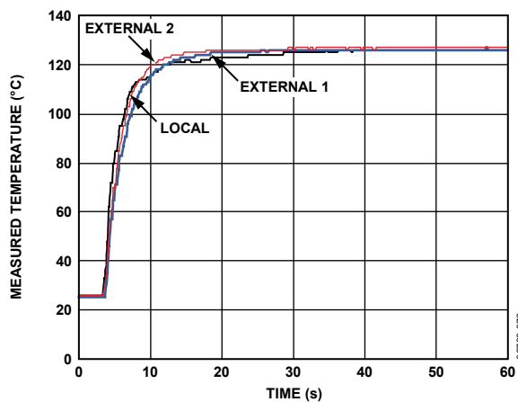
Figure 9. ADT7490 Response to Thermal Shock
