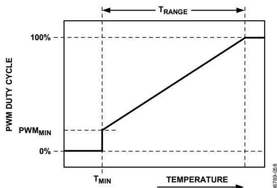
Figure 54. T RANGE Parameter Affects Cooling Slope
