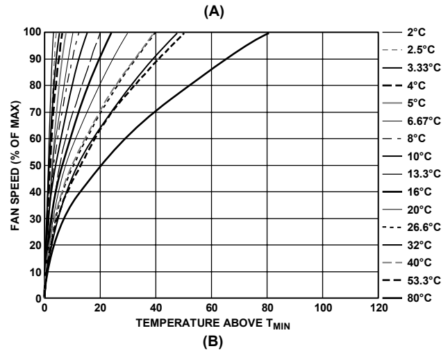
Figure 58. T_{RANGE} vs. Actual Fan Speed (Not PWM Drive) Profile
