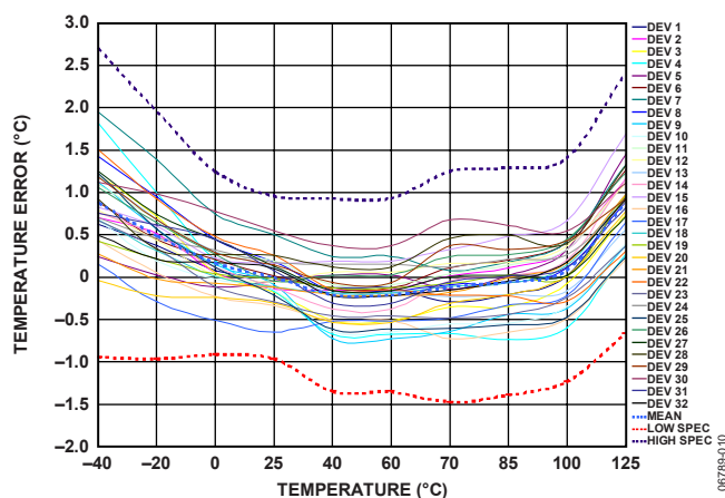
Figure 8. Remote 2 Temperature Sensor Error
