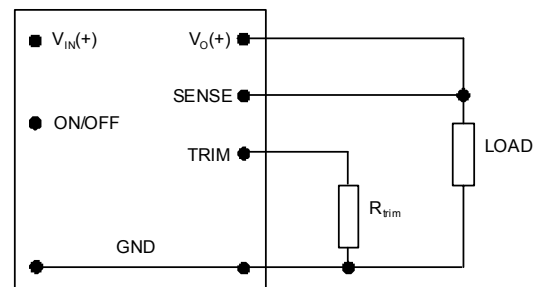
Figure 56. Circuit configuration for programming output voltage using an external resistor.
