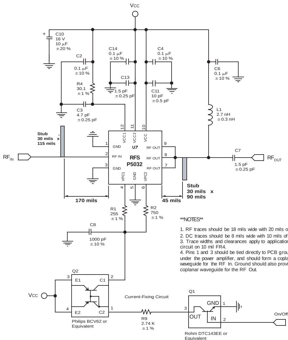
Figure 7: Application Circuit
