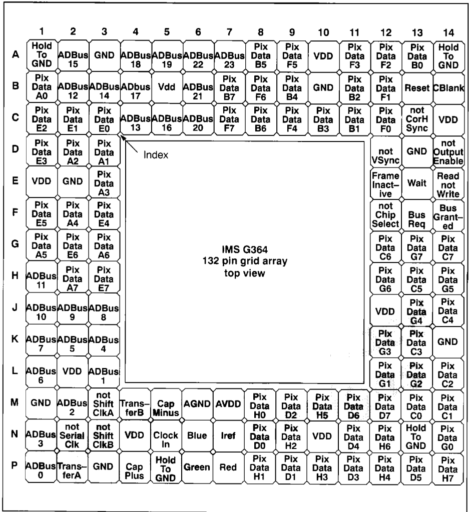
Figure 14.4 IMS G364 pin configuration
