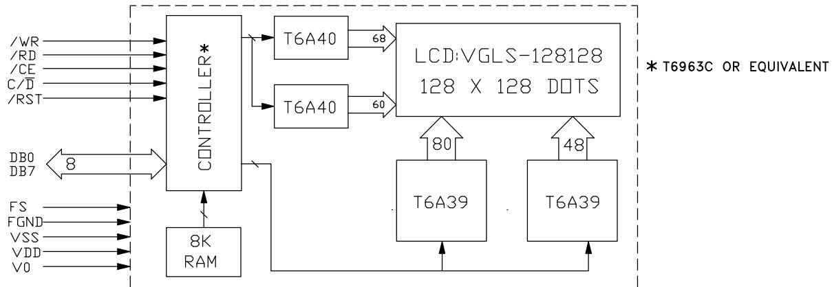
BLOCK DIAGRAM OF LCD MODULE OF MGLS128128T
