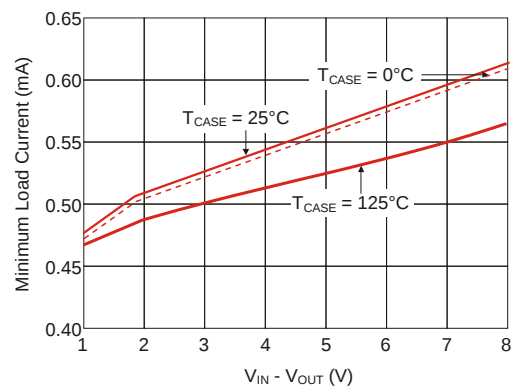
Figure 4. Minimum Load Current vs. V IN - V OUT
