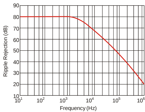
Figure 3. Ripple Rejection vs. Frequency
