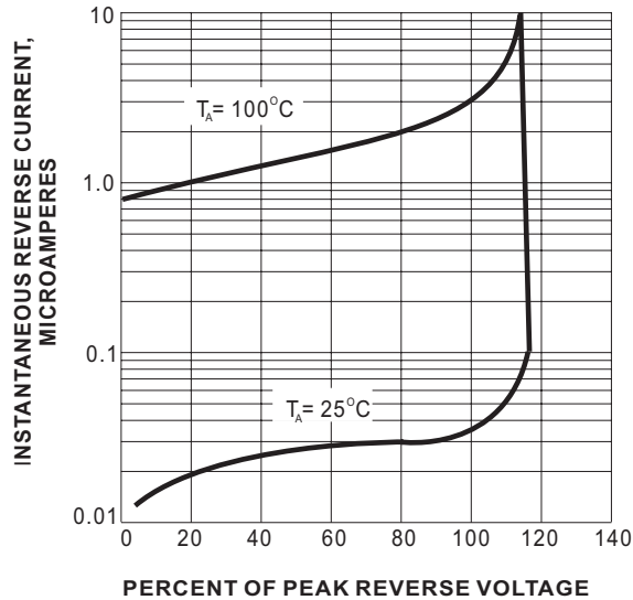
Fig. 3- TYPICAL REAK REVERSE CHARACTERISTICS
