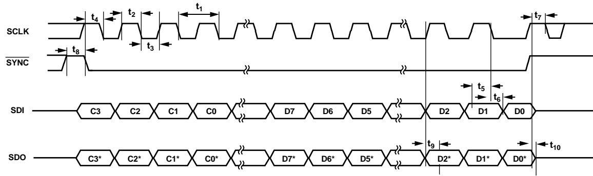
Figure 5. SPI Serial Interface Timing Diagram, CPOL = 1, CPHA = 0
