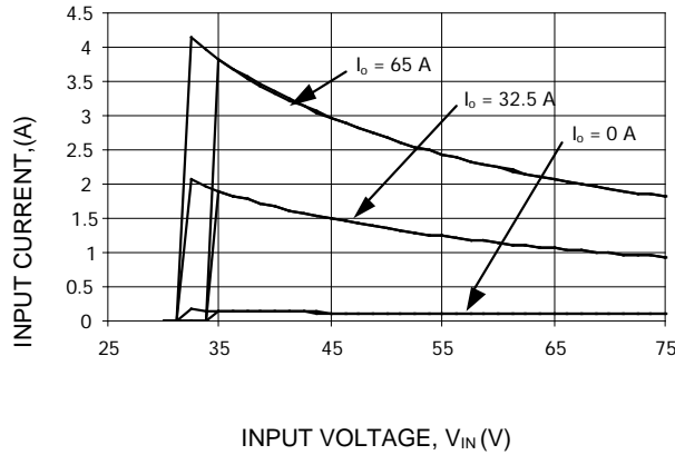
Figure 25. Typical Start-Up (Input Current) characteristics at room temperature.
