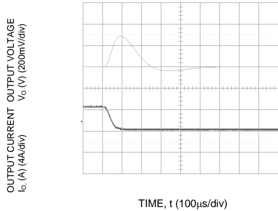
Figure 5. Transient Response to Dynamic Load Change from 50% to 25% of full load current.
