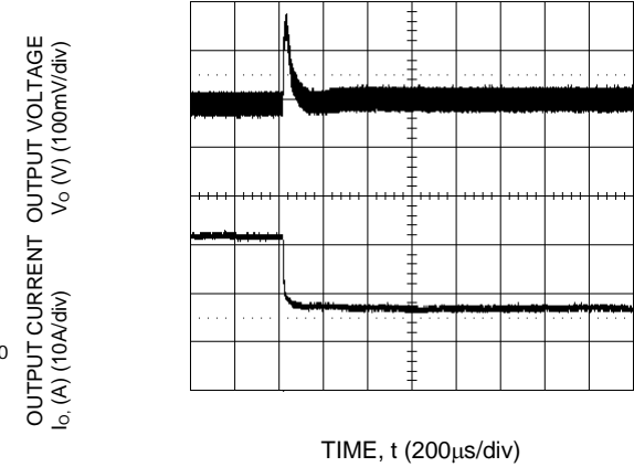
Figure 29. Transient Response to Dynamic Load Change from 50% to 25% of full load current.
