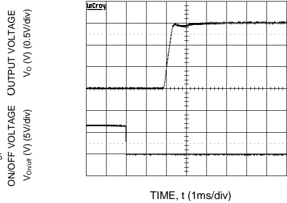
Figure 34. Typical Start-Up Characteristics from Remote ON/OFF.
