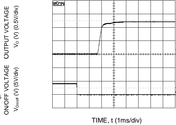
Figure 40. Typical Start-Up Characteristics from Remote ON/OFF.
