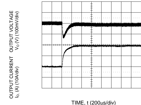
Figure 36. Transient Response to Dynamic Load Change from 25% to 50% of full load current.
