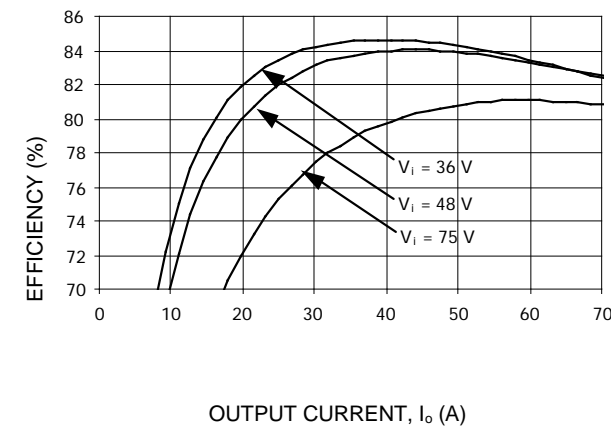
Figure 38. Converter Efficiency Vs Load at Room temperature.
