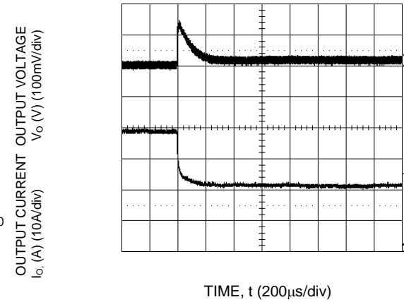
Figure 41. Transient Response to Dynamic Load Change from 50% to 25% of full load current.
