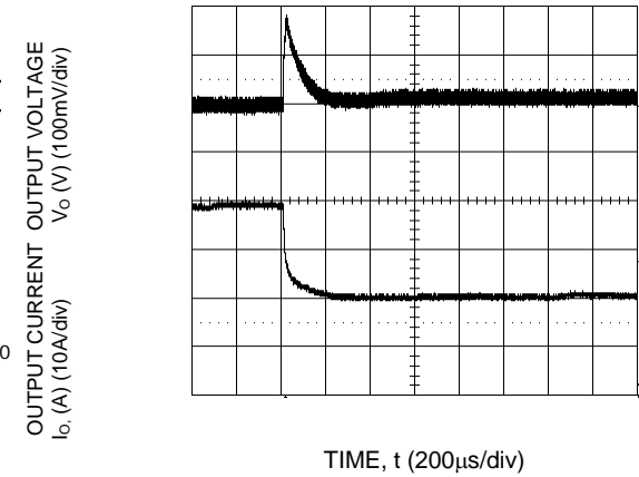
Figure 35. Transient Response to Dynamic Load Change from 50% to 25% of full load current.
