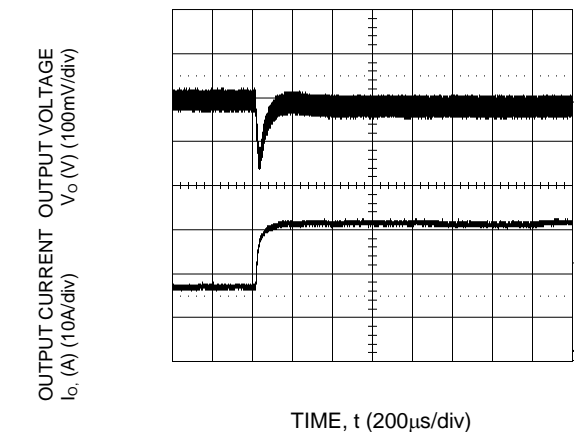
Figure 30. Transient Response to Dynamic Load Change from 25% to 50% of full load current.
