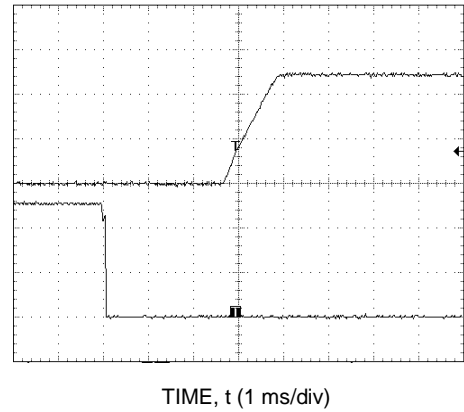
Figure 10. Typical Start-Up Characteristics from Remote ON/OFF.
