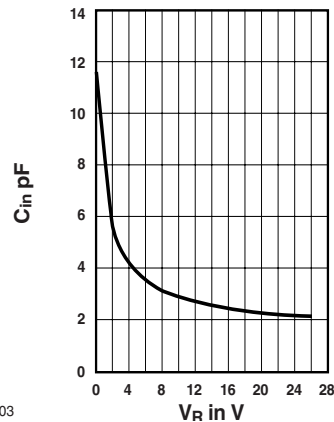
Figure 3. Typical Capacitance °C vs. Reverse Applied Voltage V R
