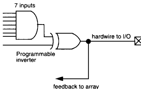
Figure 3 • D-Module Implementation
