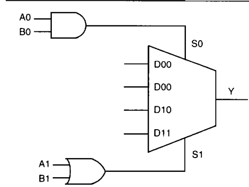
Figure 1 • C-module Implementation
