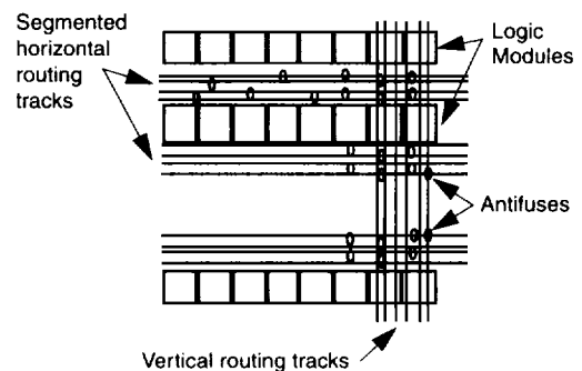
Figure 6 • Routing Structure
