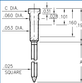
103X-X-17-XX-3X-XX-02-0 Press-fit in .057 mounting hole
