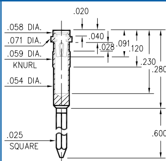
1040-3-17-XX-30-XX-02-0 Press-fit in .056 mounting hole
