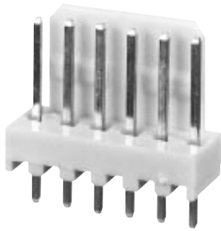
TCP-006 (shown)
