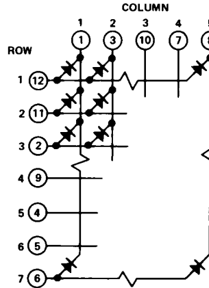
HDSP-4701/L101/L201/5401 COMMON ANODE ROW
