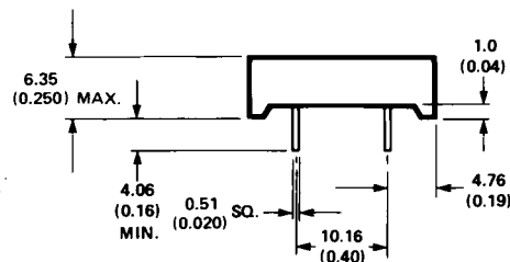
END VIEW
