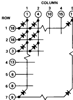
HDSP-4401/M101/4501/5101 COMMON ANODE ROW
