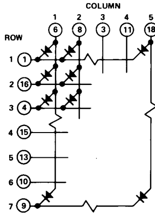
HDSP-4403/M103/4503/5103 COMMON CATHODE ROW
