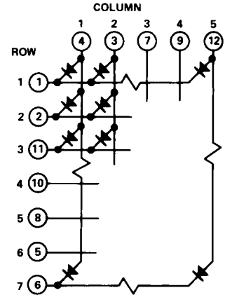
HDSP-4703/L103/L203/5403 COMMON CATHODE ROW
