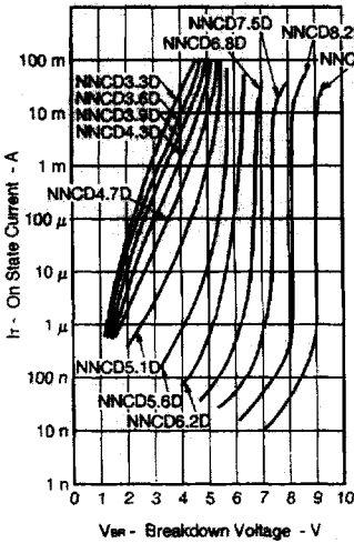
Fig. 2 I_r - V_{BR} CHARACTERISTICS
