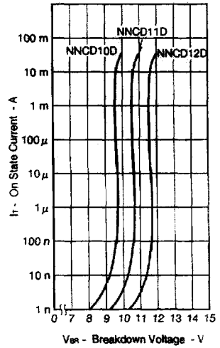
Fig. 3 I_r - V_{BR} CHARACTERISTICS
