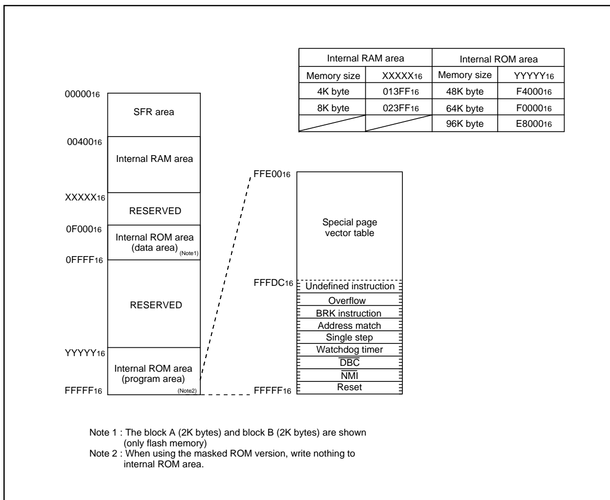
Figure 3.1. Memory Map
