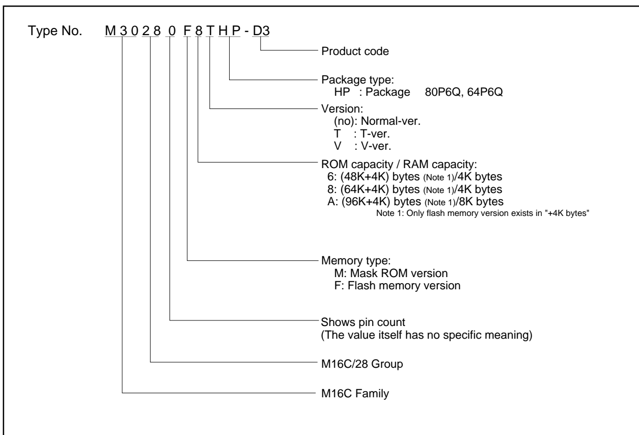
Figure 1.4.1. Type No., Memory Size, and Package
