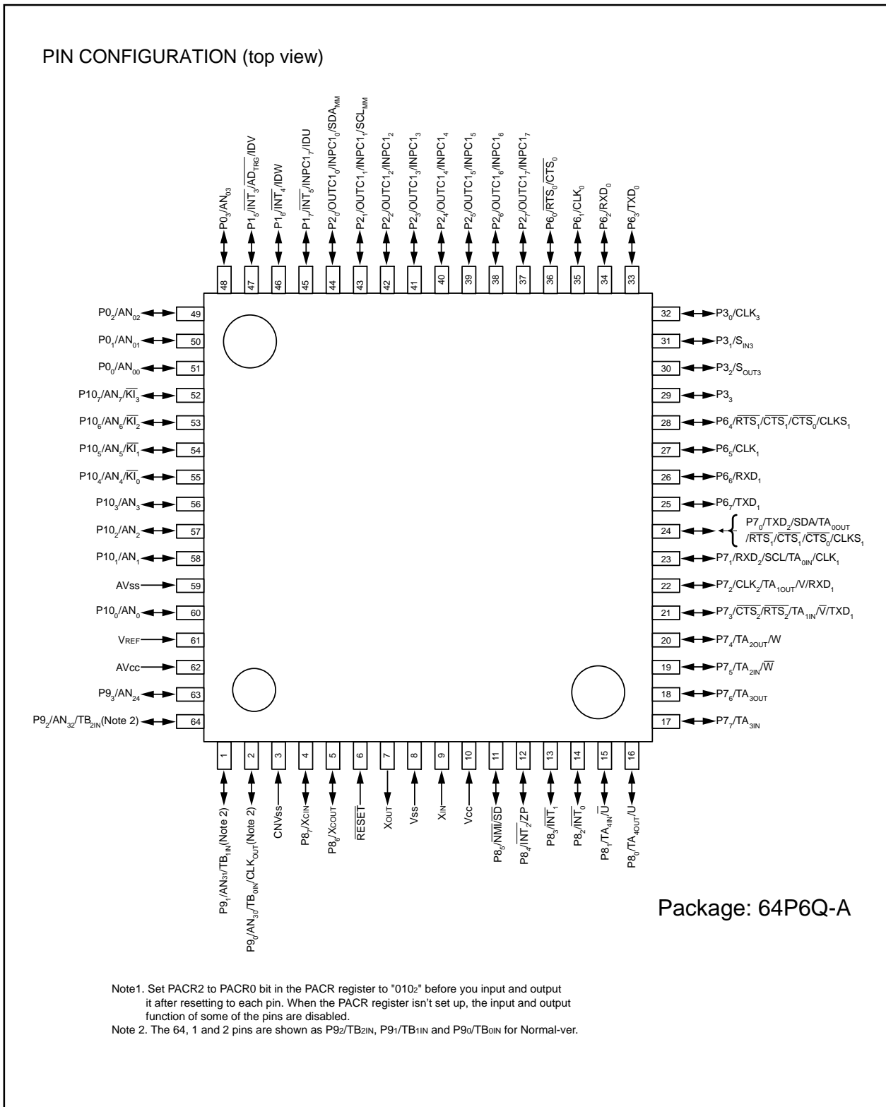
Figure 1.5.2. Pin Configuration (Top View) of M16C/28 Group, 64-pin Package
