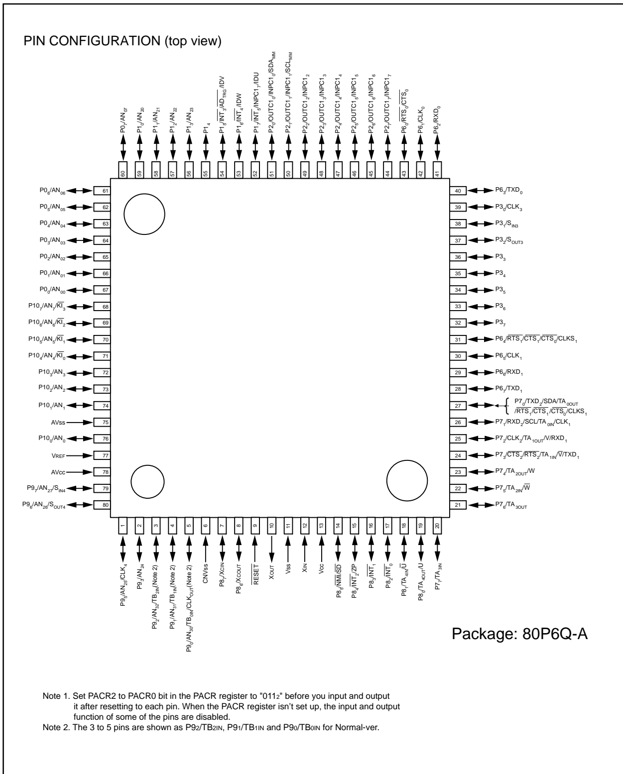
Figure 1.5.1. Pin Configuration (Top View) of M16C/28 Group, 80-pin Package
