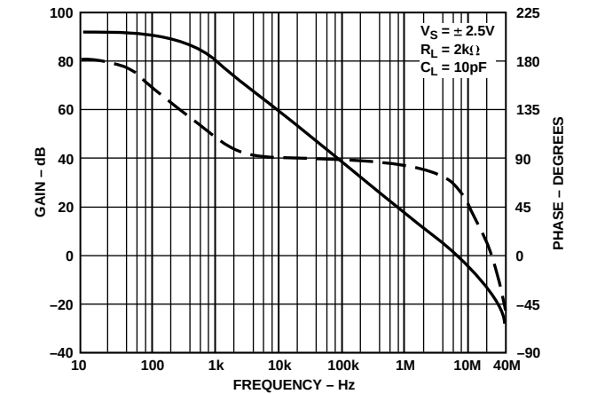
Figure 1. Phase/Gain vs. Frequency
