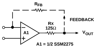
Figure 29. Output Short Circuit Protection Configuration
