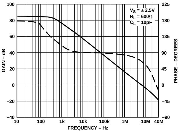
Figure 2. Phase/Gain vs. Frequency
