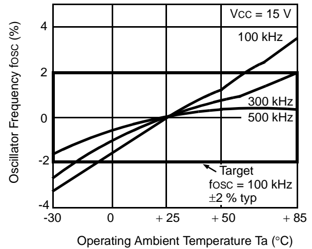
Fig. 32 -Oscillator Frequency vs. Operating Ambient Temperature
