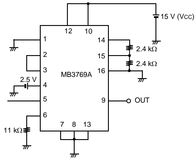
Fig. 23 -Test Circuit
