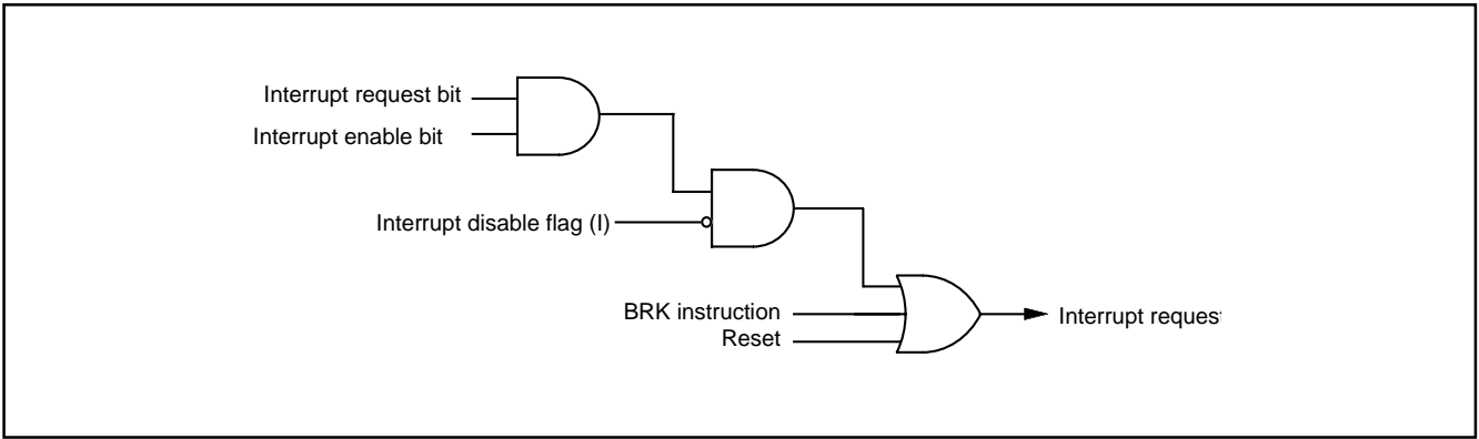
Fig. 26 Interrupt control
