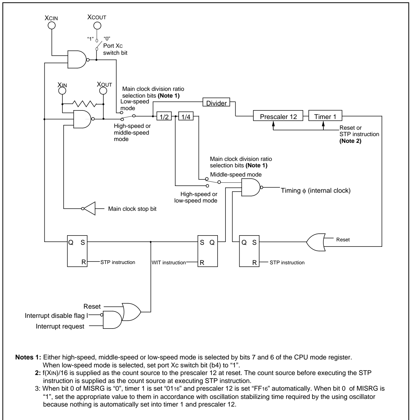
Fig. 84 System clock generating circuit block diagram (Single-chip mode)
