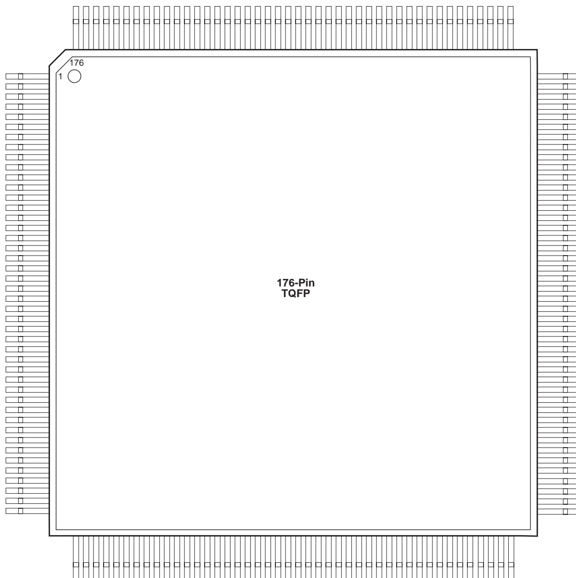
Figure 2-9 • 176-Pin TQFP
