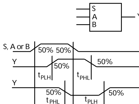
Figure 1-19 • Module Delays
