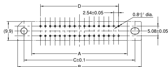
Recommended PC board pattern (Bottom view)
