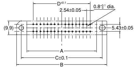
Applicable PC board dimensions
