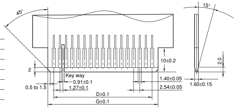
Applicable PC board dimensions
